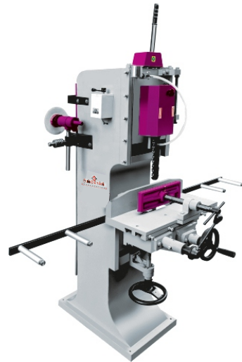
Chain/Chisel mortiser
